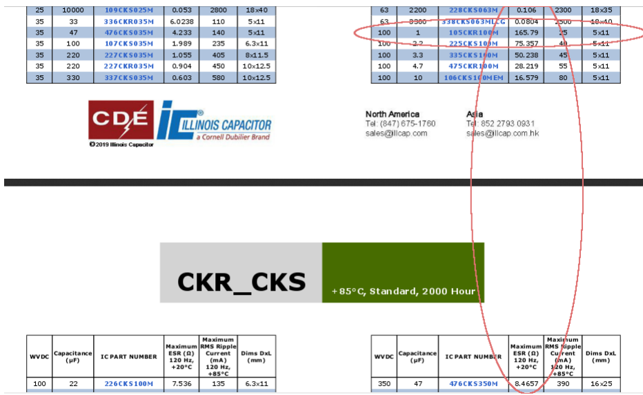
Figure 1: Notice how impedance jumps very fast with a 1uf cap, compared to the higher values. Additionally, different brands will have different impedances for a similar value cap.
