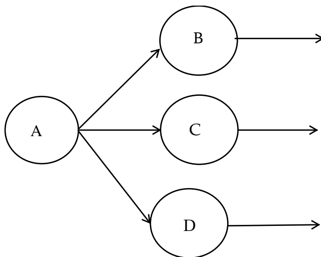
Figure 1: A Network
