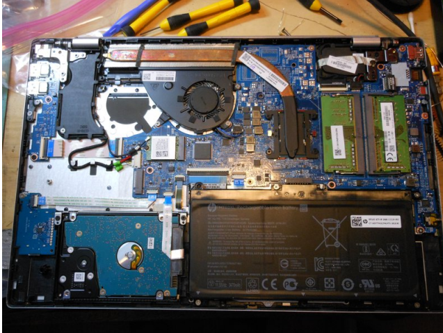
Figure 5: Disassembly
